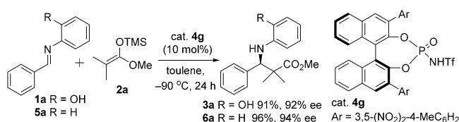
Scheme 3. Enantioselective Mukaiyama–Mannich reactions catalyzed by N -triflyl phosphoramidate 4g . Unless otherwise specified, all reactions were performed at -78^\circ\text{C} for 24 h under nitrogen with 1 (0.1 mmol, 1.0 equiv), 2a (0.3 mmol, 3.0 equiv), catalyst 4g (0.01 mmol, 10 mol%) in toluene (1 mL). Product ee values were determined by HPLC on a chiral stationary phase.
